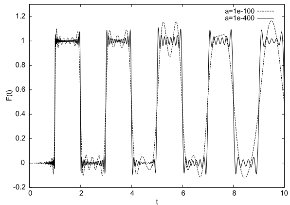
(b) \alpha = 10^{-100}, 10^{-400}
